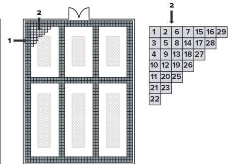
Fig. 6 Installation around fixed objects – laying tiles
