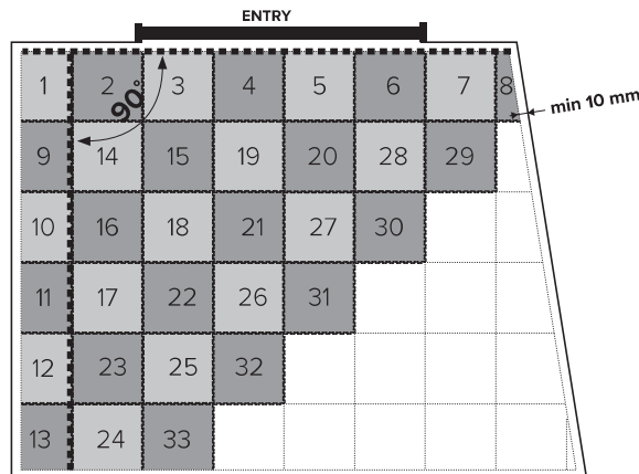
Fig. 3 Direction of installing INVISIBLE, BUSINESS
