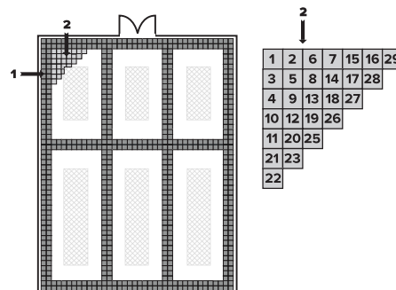
Fig. 6 Installation around fixed objects – laying tiles
